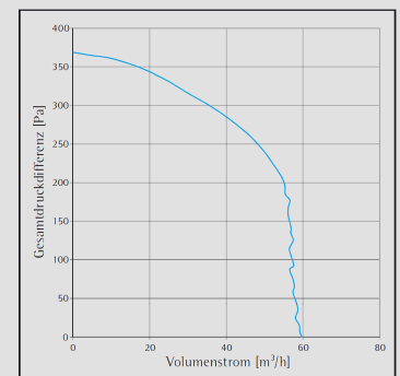
Pressure-volume characteristic curve 3/UP-2BR
